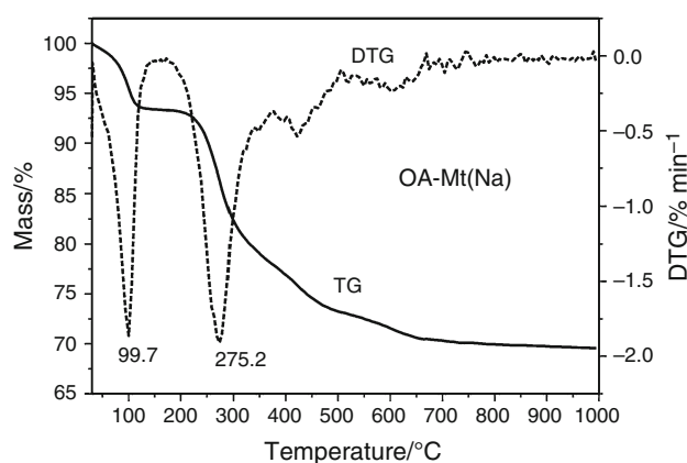
Fig. 4 TG and DTG curves for OA-Mt(Na)
